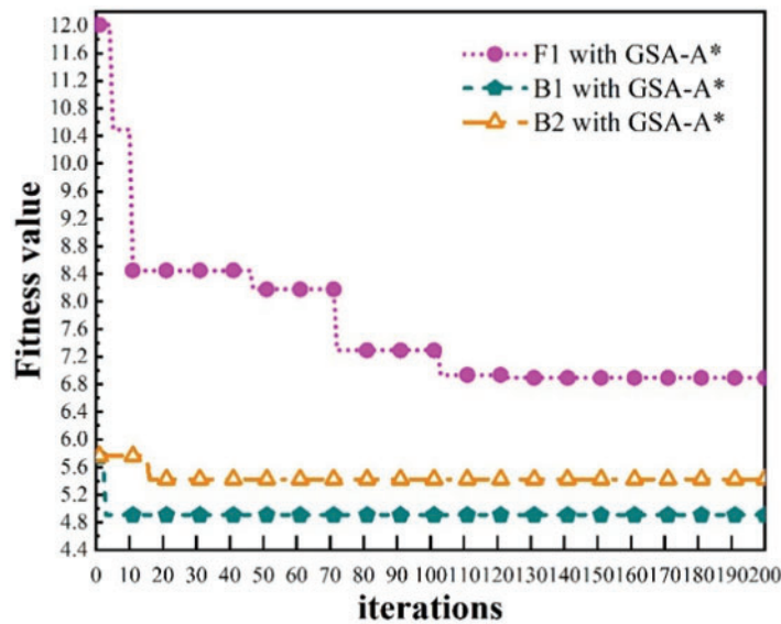
Figure 21: Comparison of fitness values (i.e., global path cost) results for GSA-A* for fire scenarios on the F1, B1, and B2 floors, respectively
