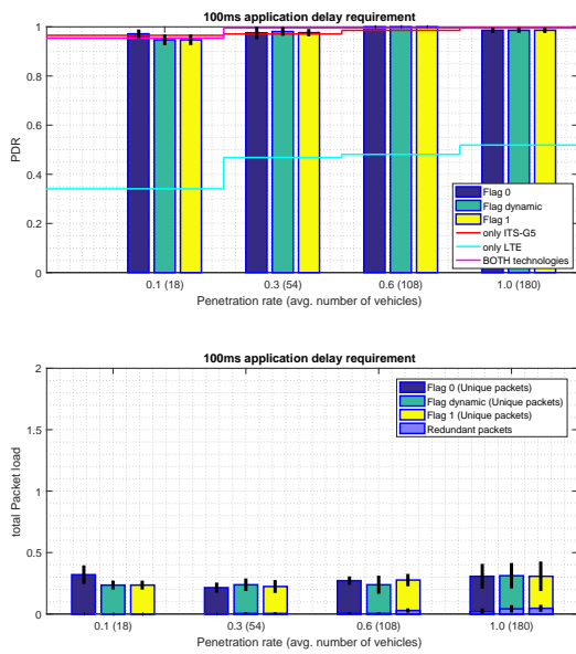
Figure 10: Upper graph: PDR; Lower graph: Total Packet load ratio for Application delay requirement 100ms (Highway scenario, close range).
