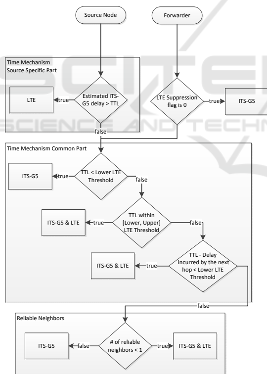
Figure 2: Algorithm flowchart.
