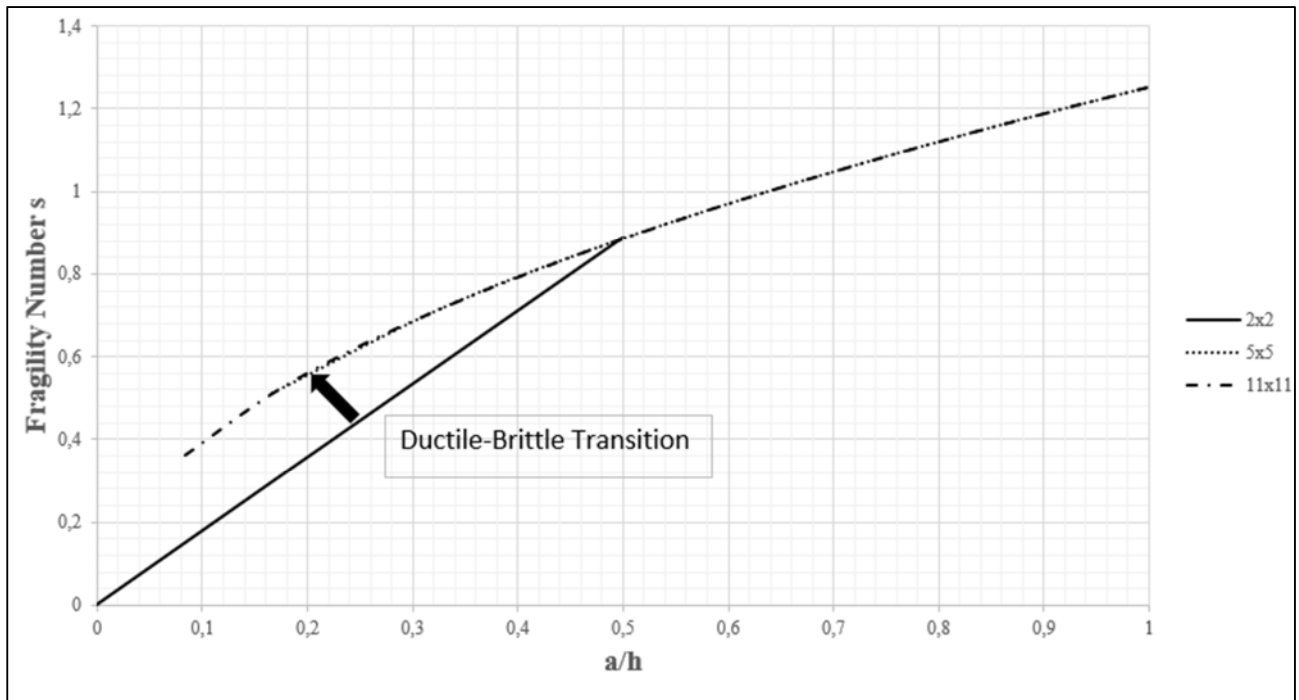
Figure 3 Transition from Ductile to Brittle behaviour in studied frames with damage CB
