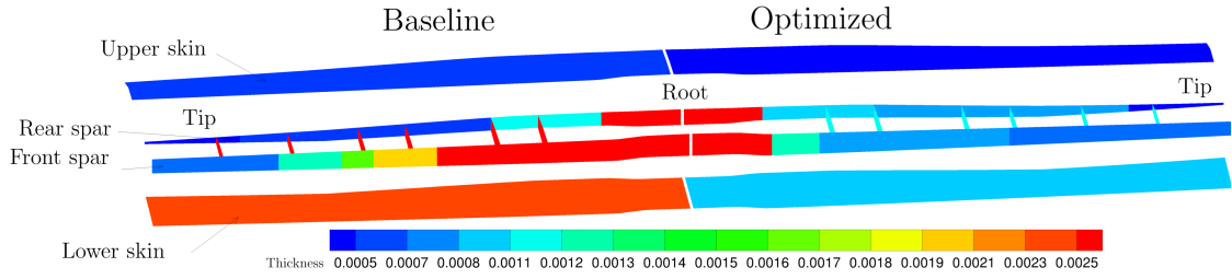
Figure 11: Thickness distribution
