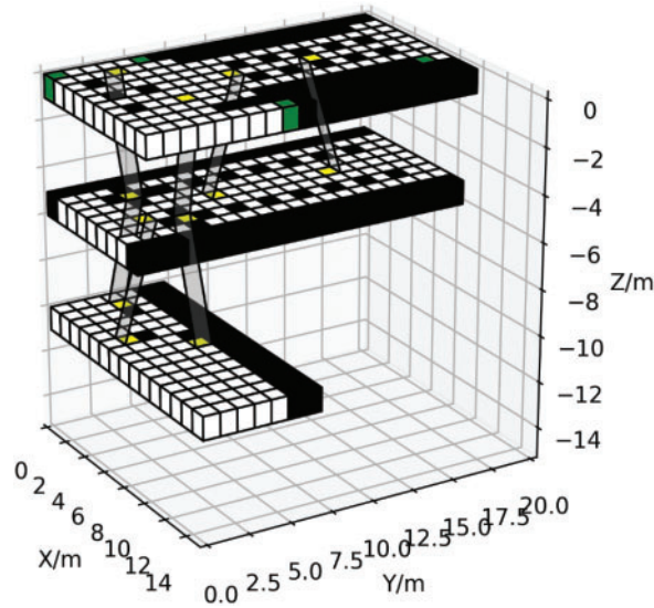
Figure 8: 3D model of Hongqi South Road Subway Station in Tianjin, China
