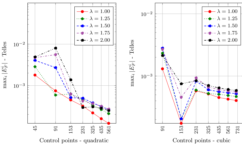
Fig. 12. Maximum error E_F^i across all angles \theta^i , for different number of control points, with quadratic NURBS (left) and with cubic NURBS (right), using Telles quadrature rules based on 8 points Gauss quadrature.
