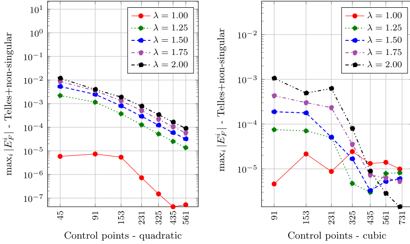
Fig. 18. Maximum error E_F^i across all angles \theta^i , for different number of control points, with quadratic NURBS (left) and with cubic NURBS (right), using Telles + non-singular quadrature rules based on 8 points Gauss quadrature.
