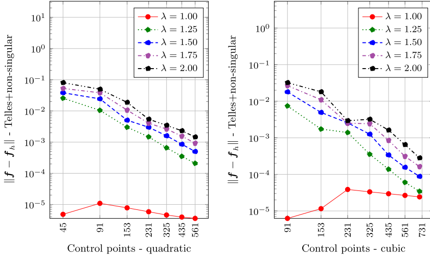
Fig. 20. L^2 error for different number of control points, with quadratic NURBS (left) and with cubic NURBS (right), using Telles + non-singular integration method, based on 8 points Gauss quadrature.
