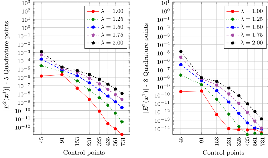
Fig. 5. Norm of E^2(\mathbf{x}^1) for 5 quadrature points (left) and for 8 quadrature points (right) for different numbers of control points.
