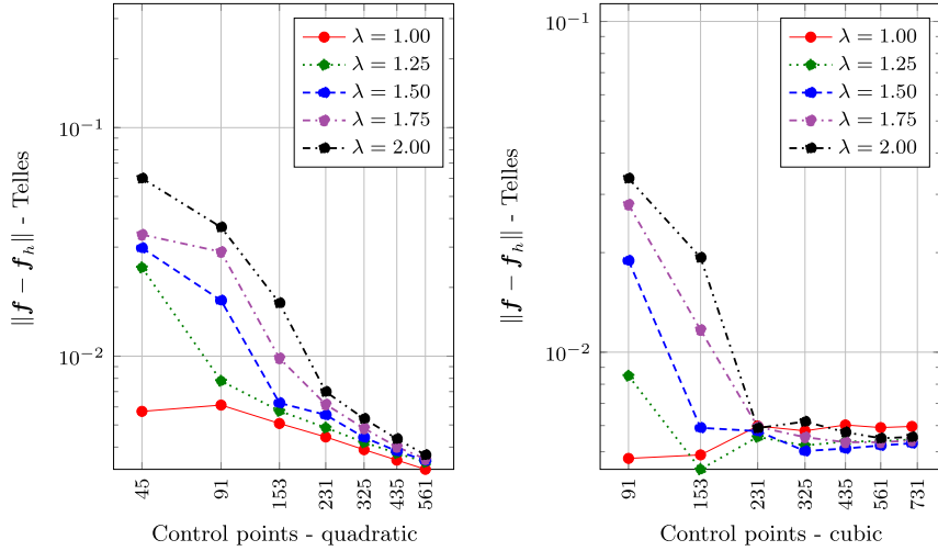
Fig. 15. L^2 error for different number of control points, with quadratic NURBS (left) and with cubic NURBS (right), using Telles integration method, based on 8 points Gauss quadrature.
