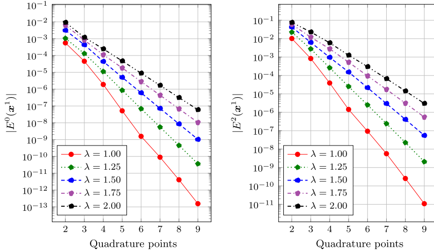
Fig. 3. Norm of E^0(\mathbf{x}^1) (left) and E^2(\mathbf{x}^1) for different numbers of quadrature points.
