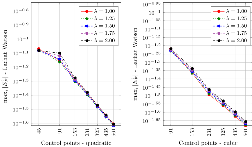
Fig. 11. Maximum error E_F^i across all angles \theta^i , for different number of control points, with quadratic NURBS (left) and with cubic NURBS (right), using Lachat Watson quadrature rules based on 8 points Gauss quadrature.
