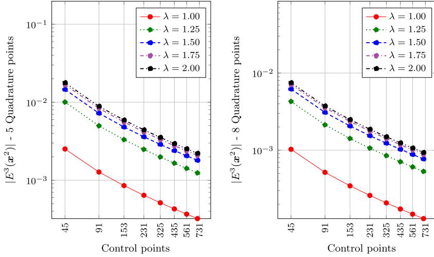
Fig. 6. Norm of E^3(\mathbf{x}^2) for 5 quadrature points (left) and for 8 quadrature points (right) for different numbers of control points.
