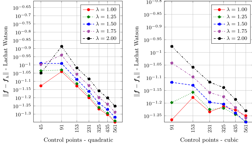
Fig. 14. L^2 error for different number of control points, with quadratic NURBS (left) and with cubic NURBS (right), using Lachat Watson integration method, based on 8 points Gauss quadrature.
