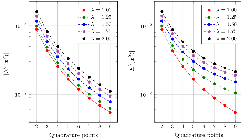
Fig. 4. Norm of E^0(\mathbf{x}^2) (left) and E^3(\mathbf{x}^2) for different numbers of quadrature points.
