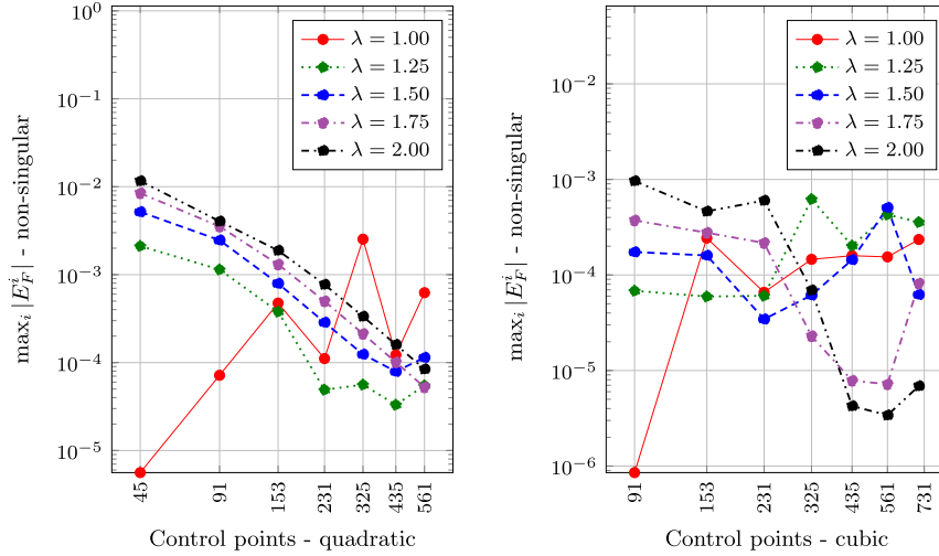
Fig. 13. Maximum error E_F^i across all angles \theta^j , for different number of control points, with quadratic NURBS (left) and with cubic NURBS (right), using non-singular quadrature rules based on 8 points Gauss quadrature.
