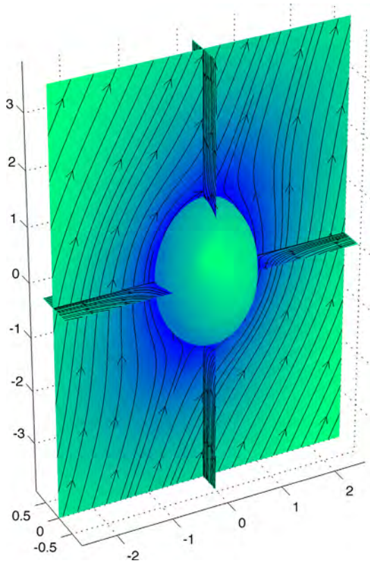
Fig. 10. Streamlines of the solution with \theta = \theta^8 and \lambda = 1.5 .
