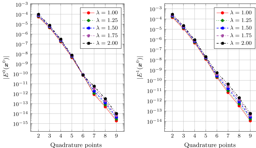
Fig. 2. Norm of E^0(\mathbf{x}^0) (left) and E^1(\mathbf{x}^0) for different numbers of quadrature points.
