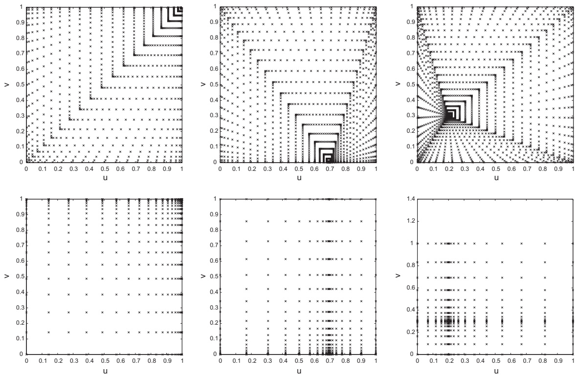
Fig. 8. Singular quadrature formulas based on Lachat-Watson (top) and Telles transformations (bottom) for singularities on the points (1,1) (left), (0.7,0) (center), and (0.2,0.3) (right), based on equi-spaced quadrature rules with 21 \times 21 points.
