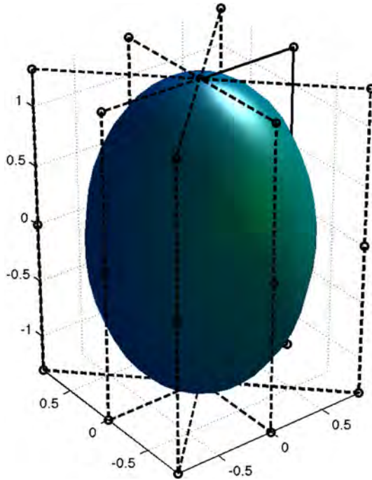
Fig. 1. Control net and NURBS surface of a prolate spheroid with ratio \lambda = 1.5 .
