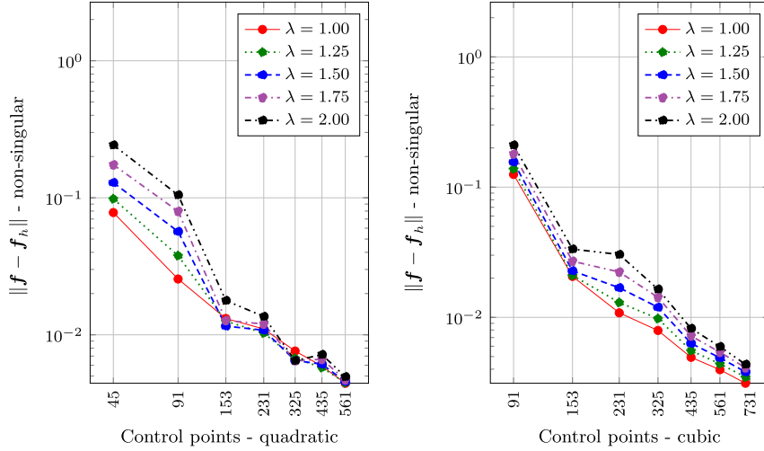
Fig. 16. L^2 error for different number of control points, with quadratic NURBS (left) and with cubic NURBS (right), using non-singular integration method, based on 8 points Gauss quadrature.
