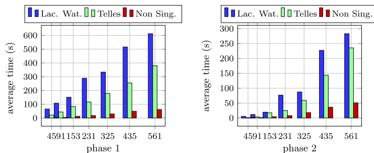
Fig. 9. Average cost between standard IGA-BEM and non-singular IGA-BEM for 8 quadrature points.
