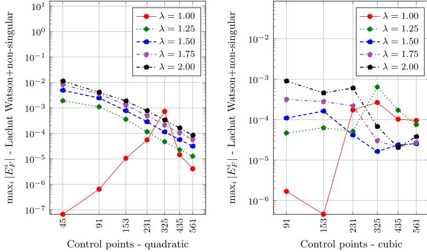
Fig. 17. Maximum error E_F^i across all angles \theta^i , for different number of control points, with quadratic NURBS (left) and with cubic NURBS (right), using LachatWatson + non-singular quadrature rules based on 8 points Gauss quadrature.
