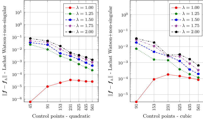
Fig. 19. L^2 error for different number of control points, with quadratic NURBS (left) and with cubic NURBS (right), using Lachat Watson + non-singular integration method, based on 8 points Gauss quadrature.
