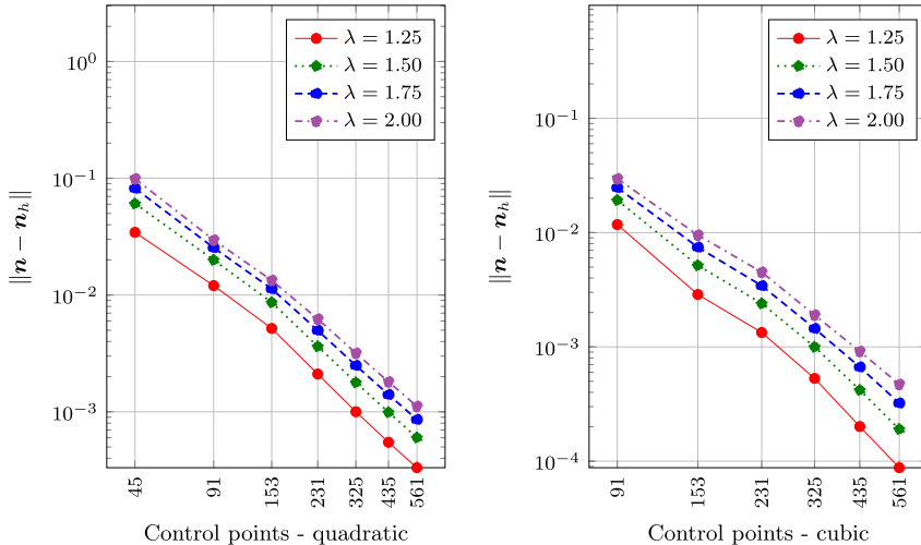
Fig. 7. L^2 error in the representation of the normal \mathbf{n} for different number of control points, with quadratic NURBS (left) and with cubic NURBS (right), based on standard 8 points Gauss quadrature rules. Increasing the number of quadrature points does not improve the graph any further.
