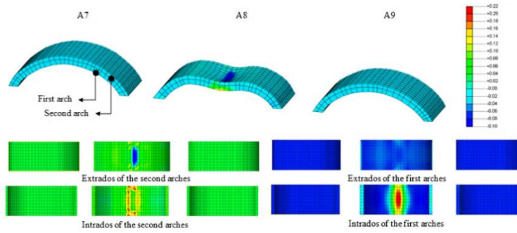
Figure 10: Failure mechanism obtained from the 'middle-span' loading performed for G_{fI}^I=0.01 N/mm with the presentation of maximum principal stresses (Scale: -0.10/+0.22 N/mm 2 ).
