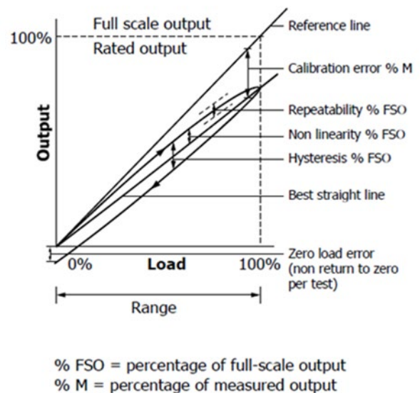
Figure 1. Definition of calibration characteristics (from Schaap and Zuidberg 1982, as presented in Lunne et al 1997)
