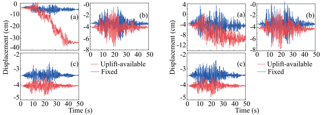
Fig. 13: Target displacements of gantry crane in Case 1 for 2%, 10%, 63% seismic excitations in trolley-travel direction Fig. 14: Target displacements of gantry crane in Case 1 for 2%, 10%, 63% seismic excitations in cart-travel direction
